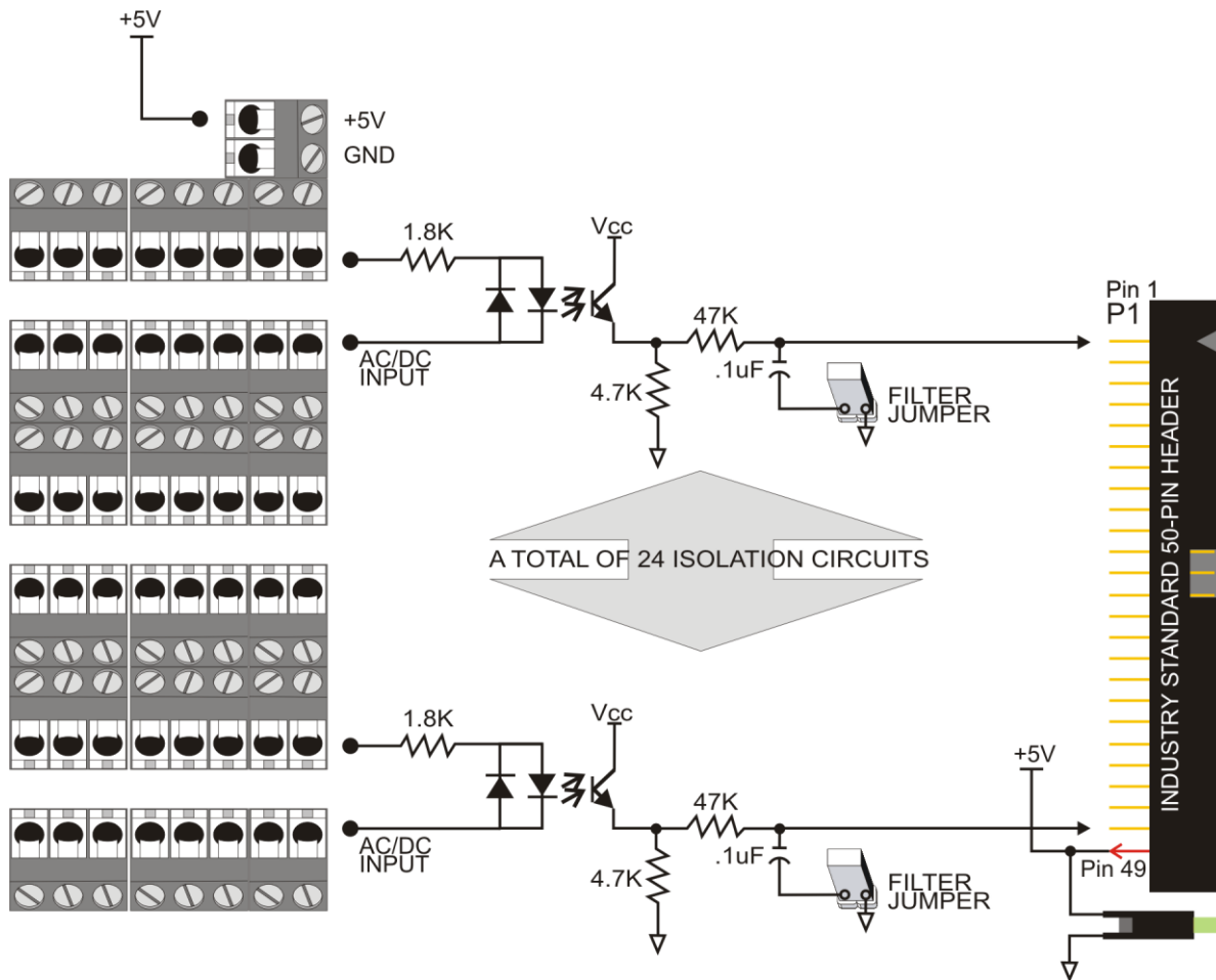
BLOCK DIAGRAM
